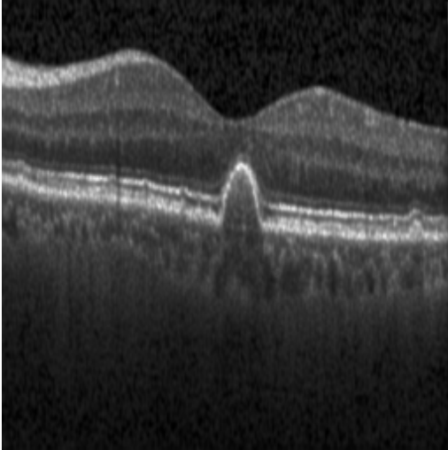
reconstruction_0.png
