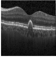
variation_0.png
