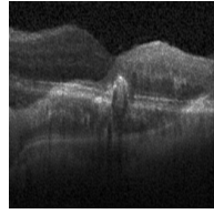
variation_2.png
