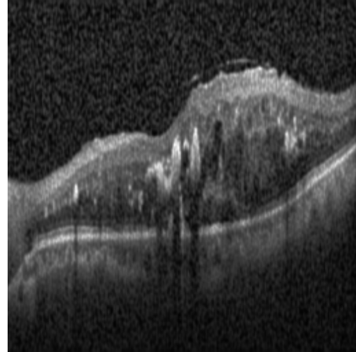
reconstruction_1.png
