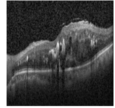
variation_4.png
